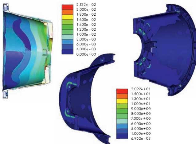
钟形罩的强度计算 Strength calculation of a bellhousing
